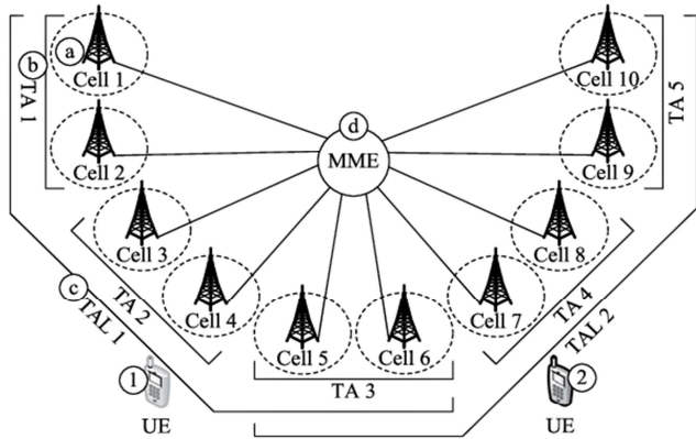
Figure 1. TAL structure in LTE.
